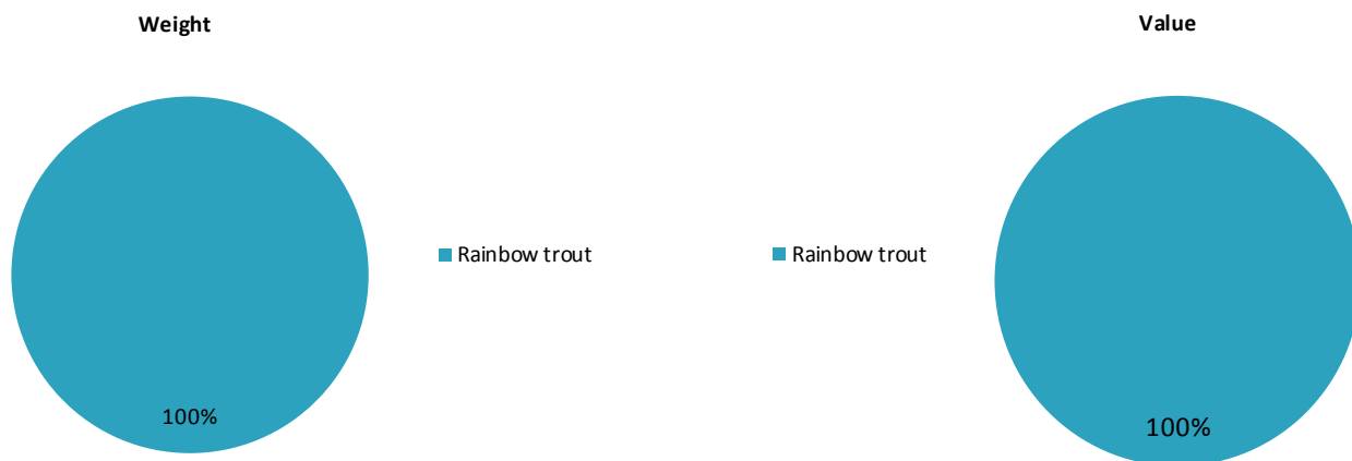
Figure 4.2.1 Main species in terms of weight and value in Belgian production: 2011.
